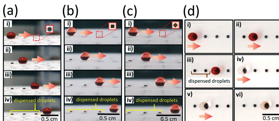
Fig. 7 Droplet dispensing from a large droplet (volume = 10 \mu\text{L} ): (a) A small red droplet is dispensed on each circular dot hydrophilic symbol. While a large droplet moves over the hydrophilic dots, each symbol attracts the droplet and a small volume is left on each symbol. (b) Small red droplets are dispensed on rectangular-shaped hydrophilic symbols. (c) Small red droplets are dispensed on diamond-shaped hydrophilic symbol. (d) After the dispensing operation on circular dot symbols, a clear water droplet is transported across the dot symbols, causing the red colour intensity to increase in the clear droplet. Scale bar = 0.5 cm.
