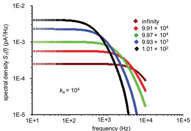
Fig. 6. The spectral density of particle number fluctuations obtained from Eq. (14) with fixed k_a = 10^4 and values of k_d varying from bottom to top: infinity (free diffusion), 9.91 \times 10^4 , 9.97 \times 10^4 , 9.93 \times 10^3 and 1.01 \times 10^2 .
